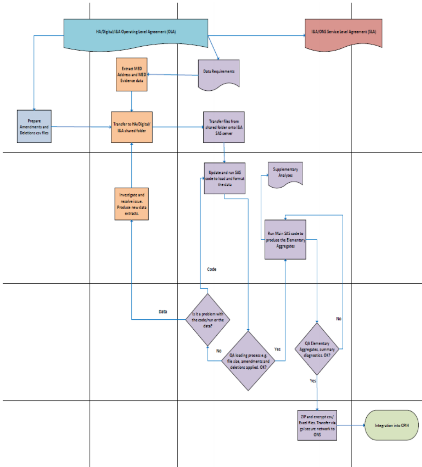
Figure 2: VOA data flow diagram – OOH processing
